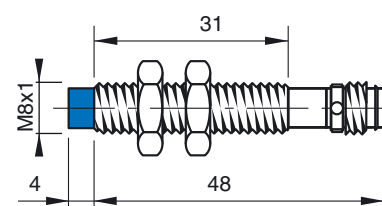
CONFIGURATION WITH CONNECTOR K1
