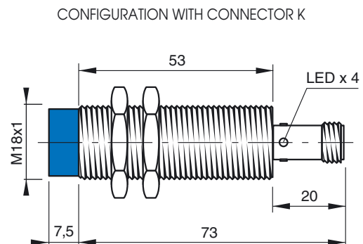
CONFIGURATION WITH CONNECTOR K
